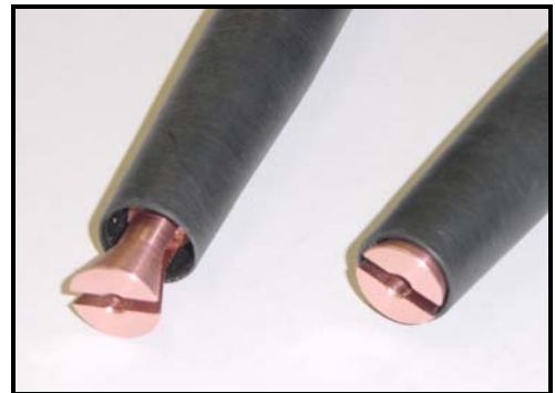
CLOSE-UP VIEW OF HIGH CONDUCTIVITY COPPER CONNECTION ENDS
